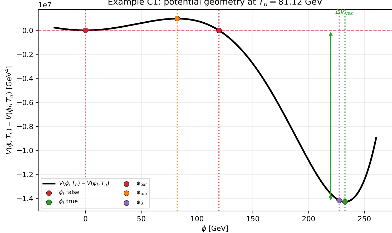
Example C1: potential geometry at T_n = 81.12 GeV
