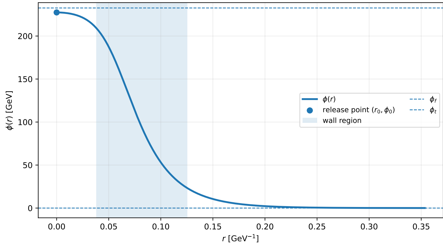
Example C3: bounce profile at T_n = 81.12 GeV
