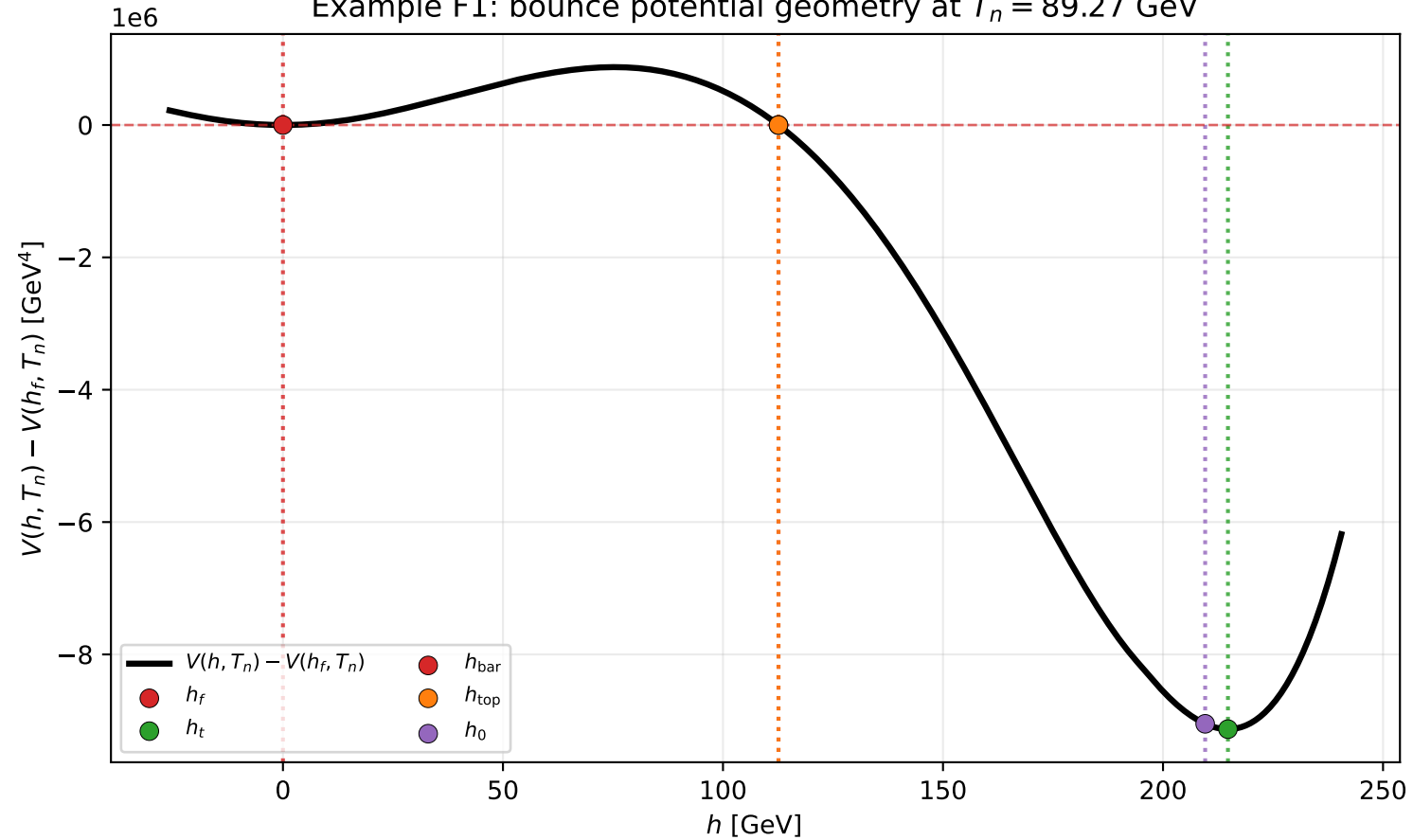
Example F1: bounce potential geometry at T_n = 89.27 GeV
