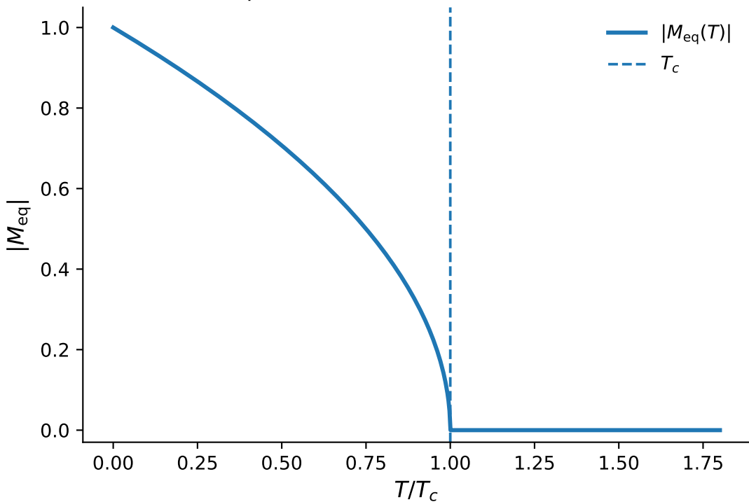
Order parameter in a continuous transition
