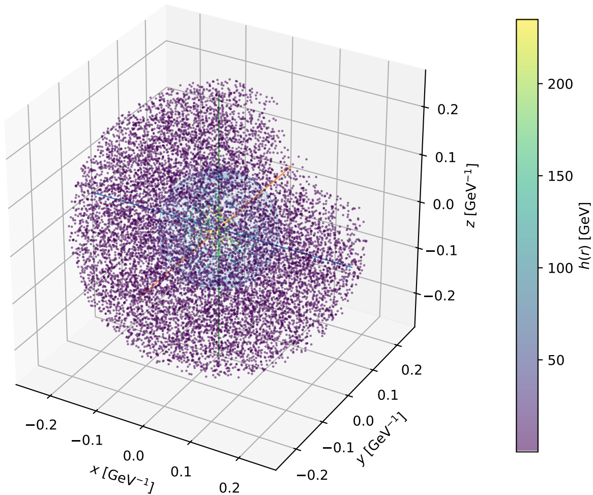
Example F5: 3D bubble profile at T_n = 70 GeV
