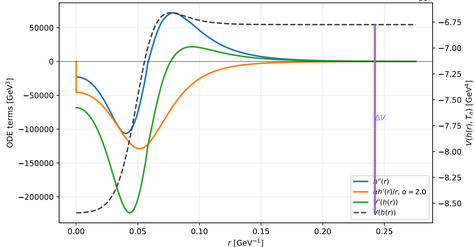
Example F7: bounce equation terms at T_n = 70 GeV
