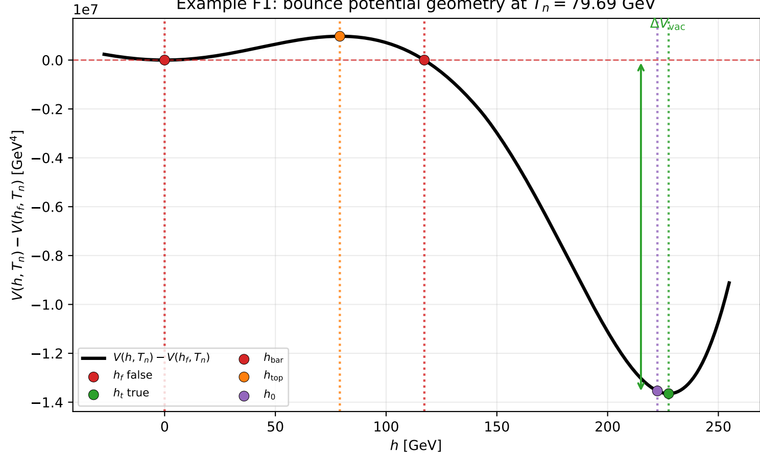
Example F1: bounce potential geometry at T_n = 79.69 GeV
