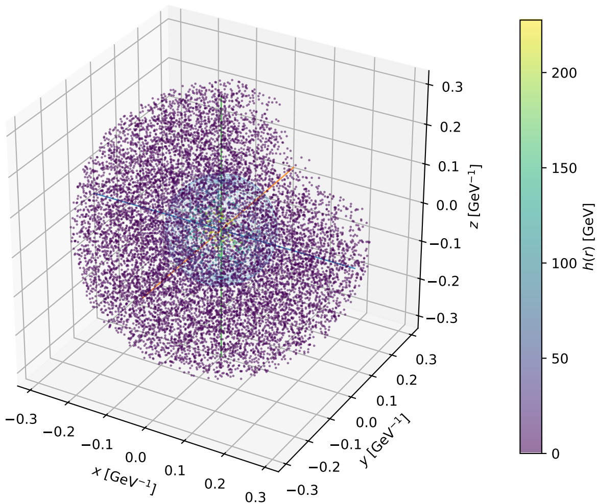
Example F5: 3D bubble profile at T_n = 79.69 GeV
