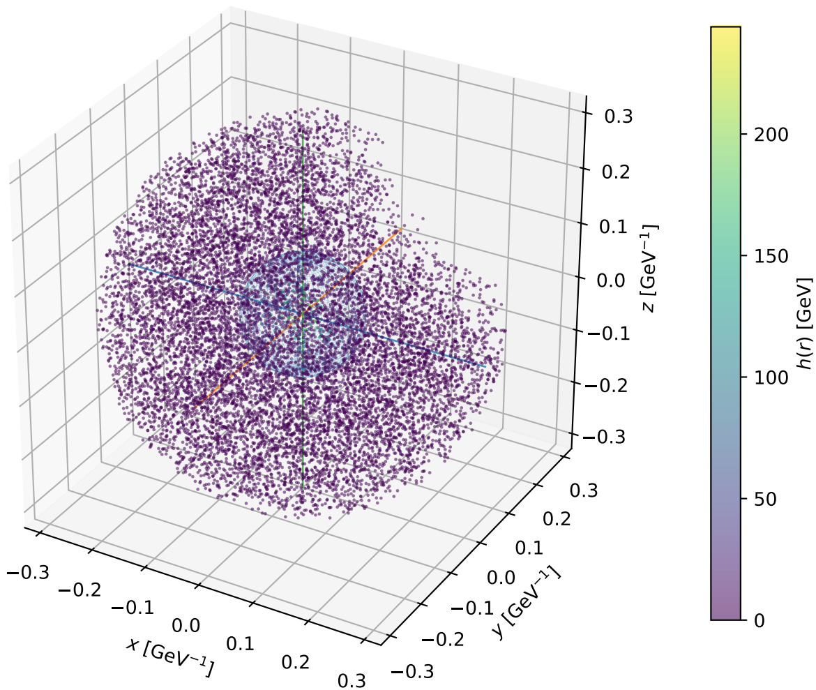
Example F5: 3D bubble profile at T_n = 42.77 GeV
