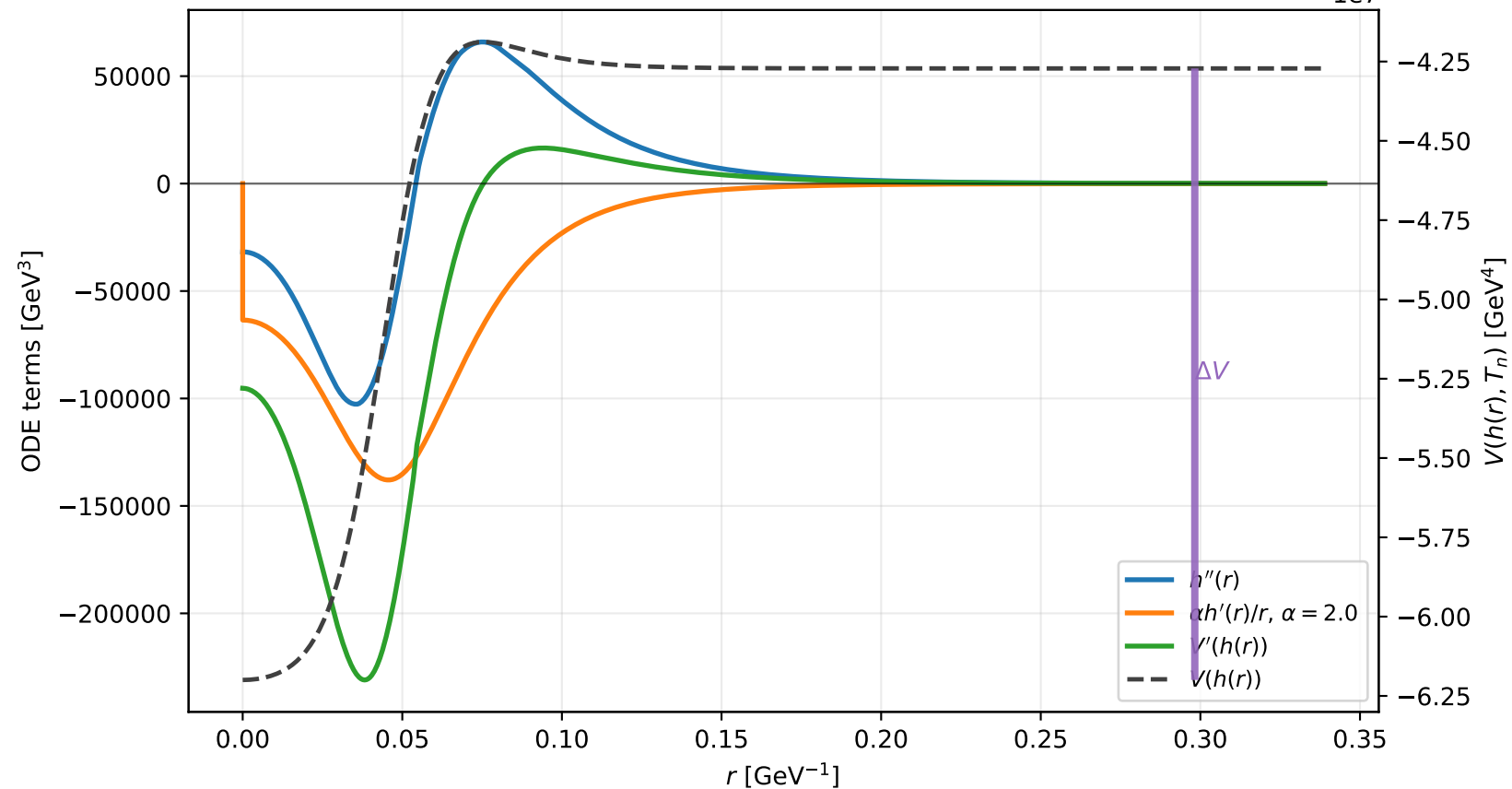
Example F7: bounce equation terms at T_n = 62.03 GeV
