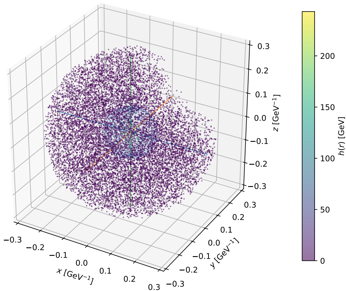
Example F5: 3D bubble profile at T_n = 47.65 GeV
