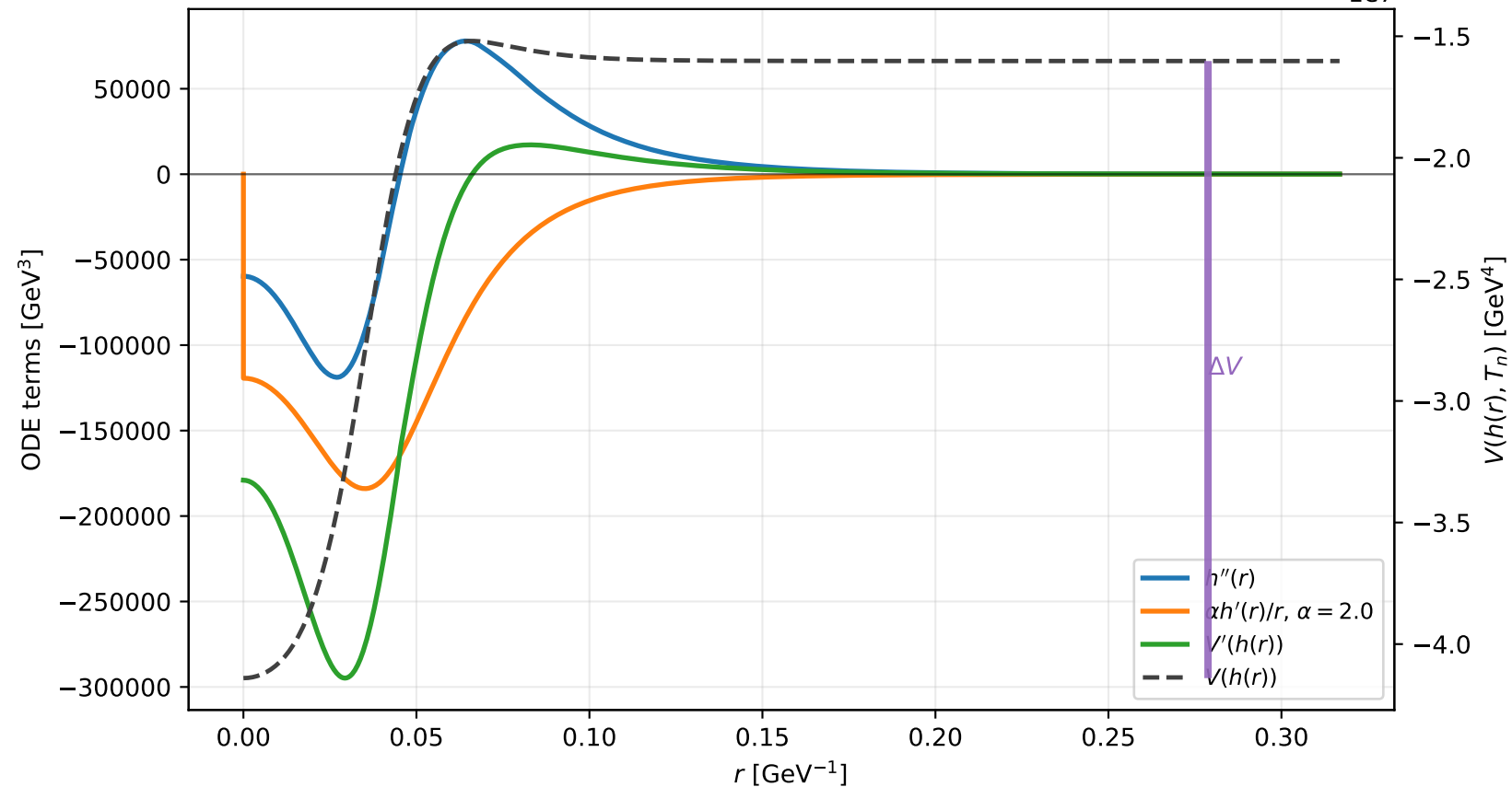
Example F7: bounce equation terms at T_n = 47.65 GeV
