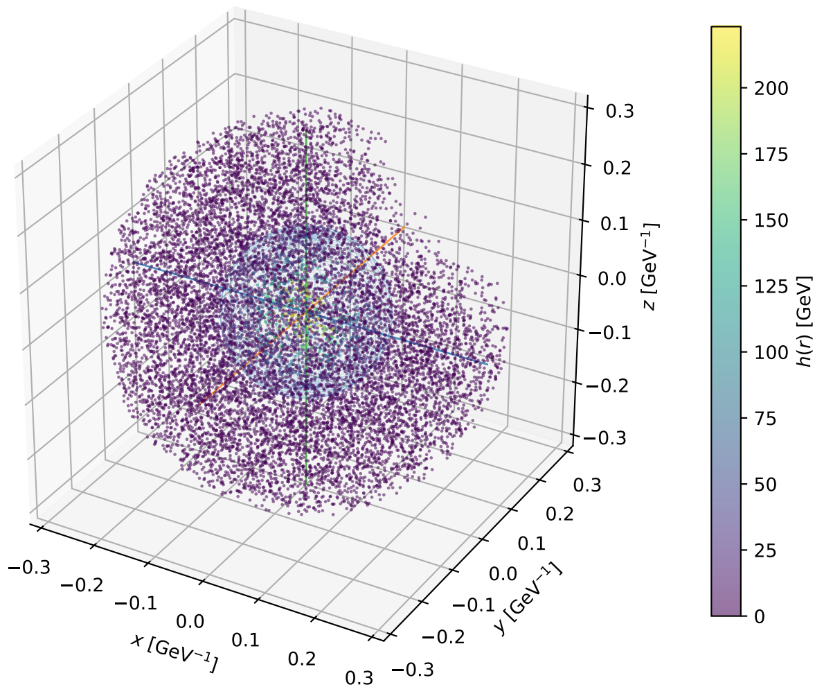
Example F5: 3D bubble profile at T_n = 83.83 GeV
