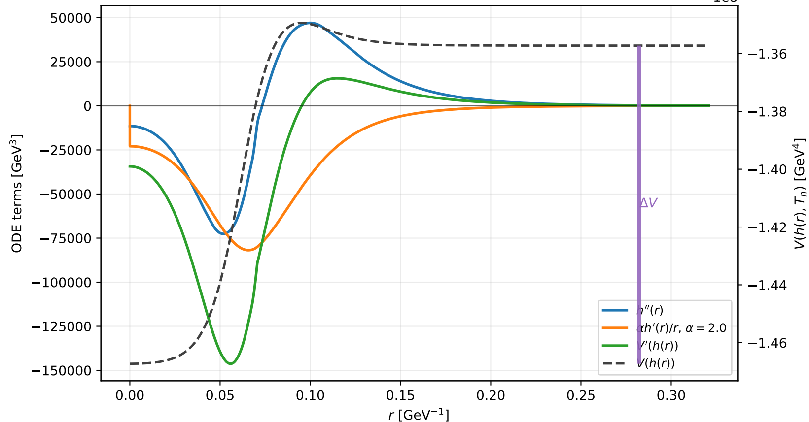
Example F7: bounce equation terms at T_n = 83.83 GeV
