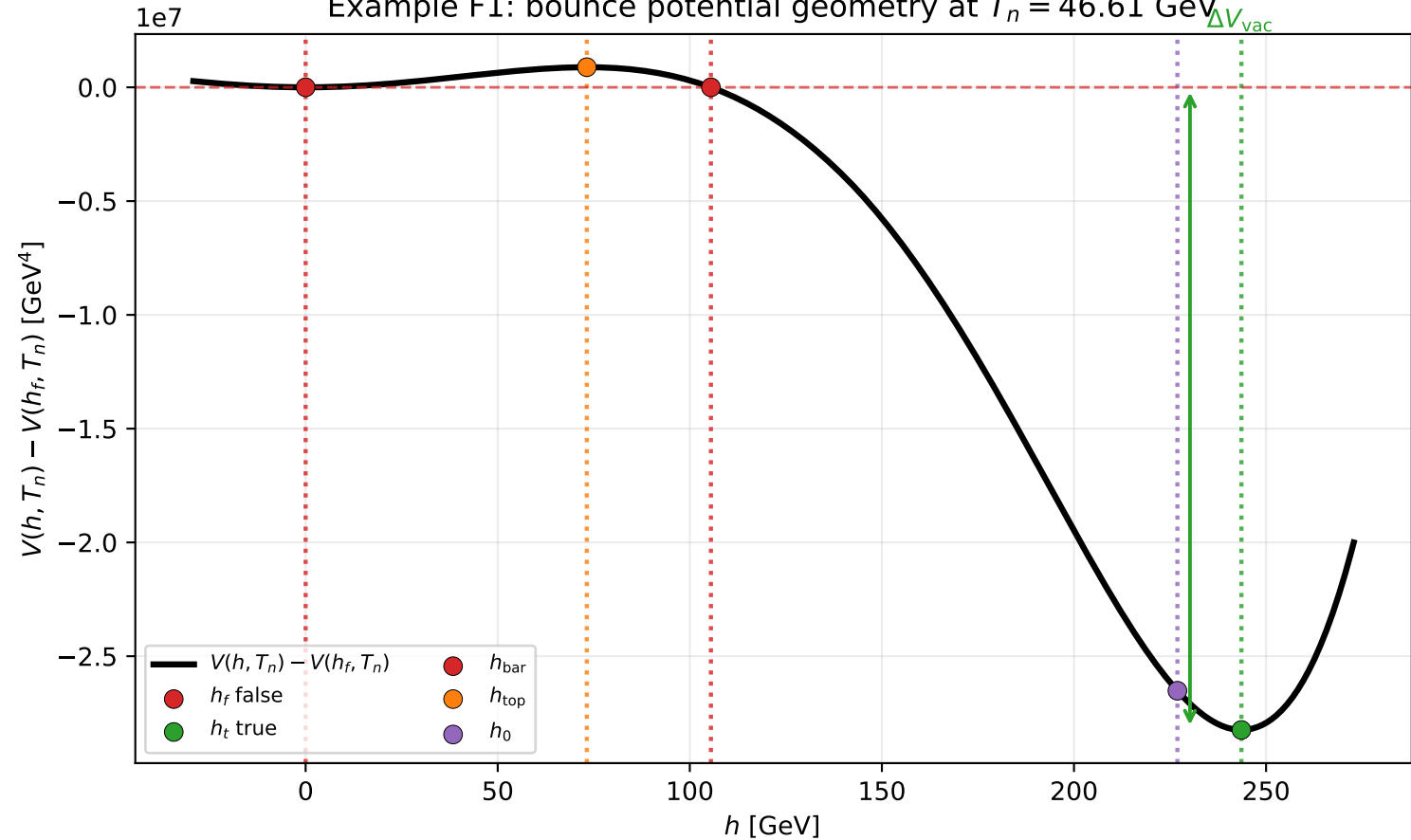
Example F1: bounce potential geometry at T_n = 46.61 GeV
