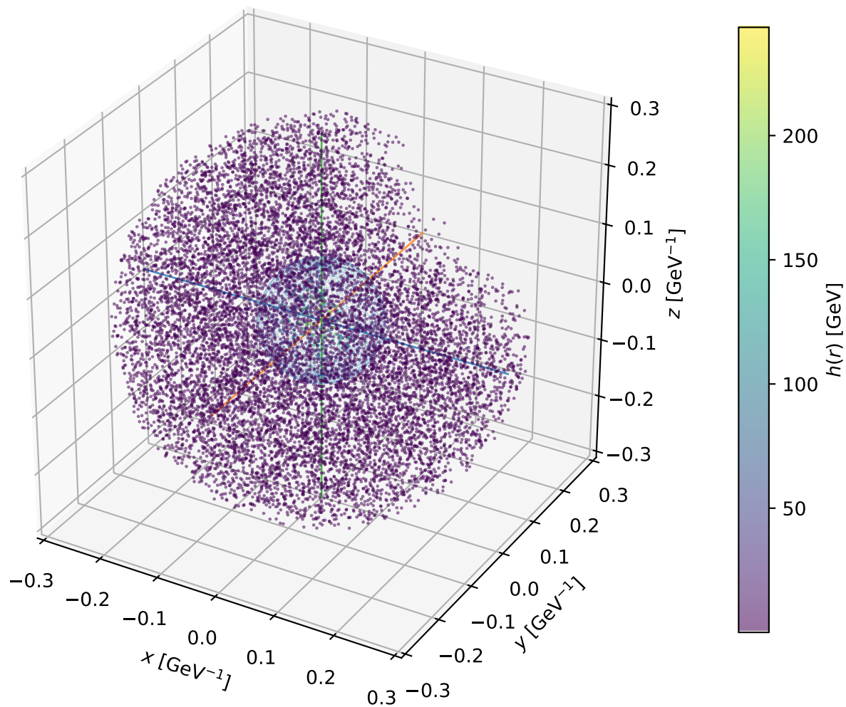
Example F5: 3D bubble profile at T_n = 46.61 GeV
