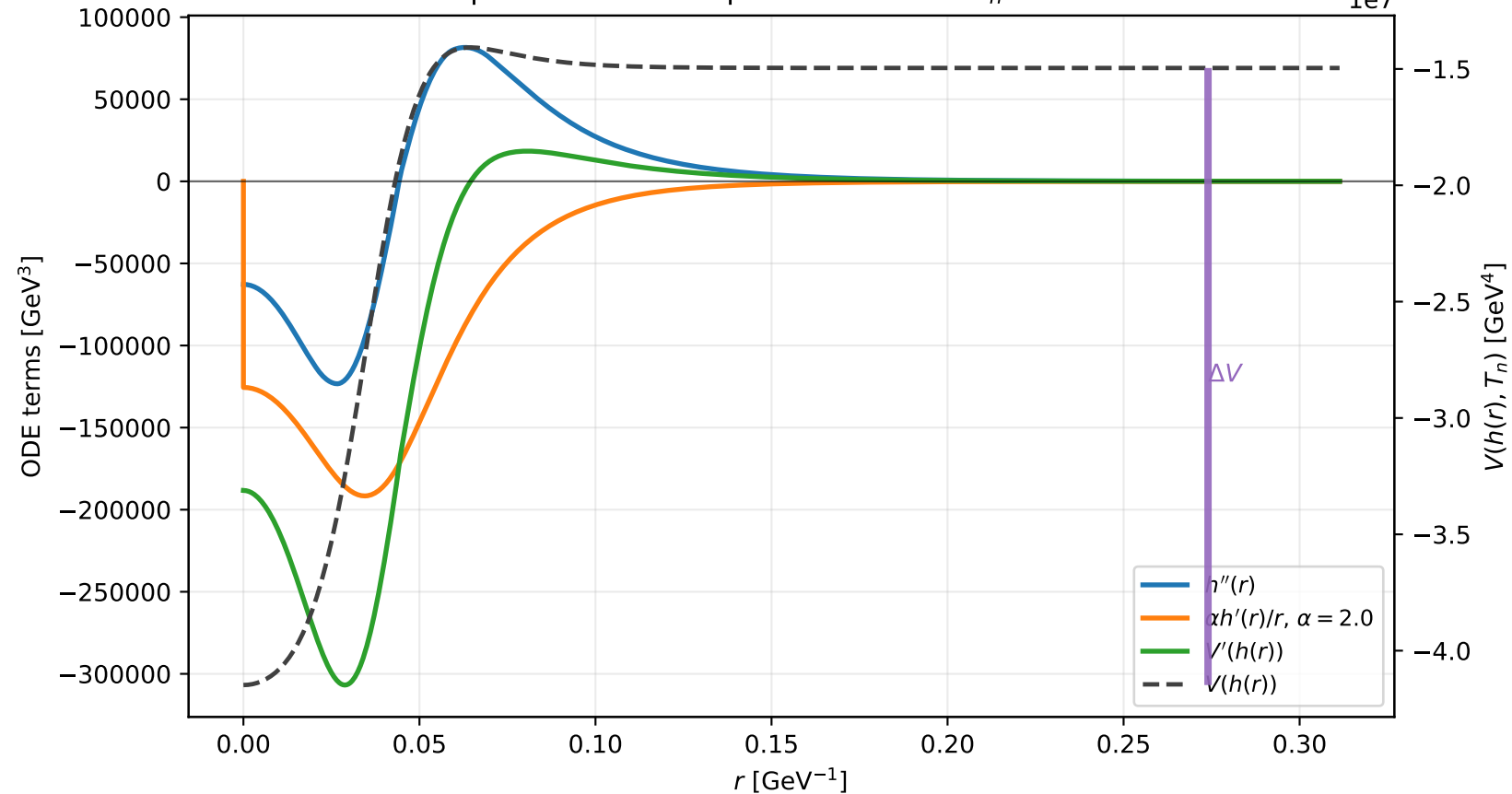
Example F7: bounce equation terms at T_n = 46.61 GeV
