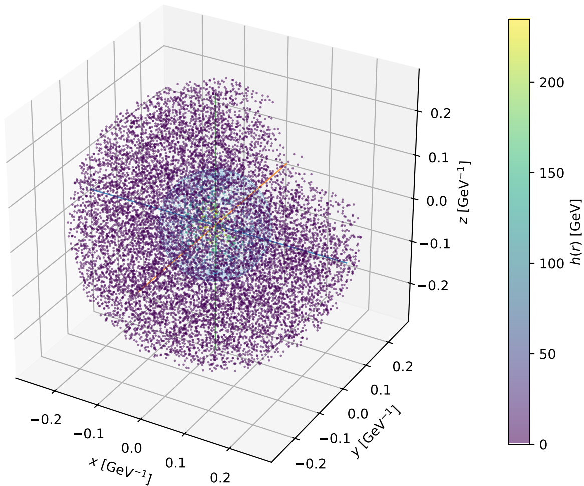
Example F5: 3D bubble profile at T_n = 71.17 GeV
