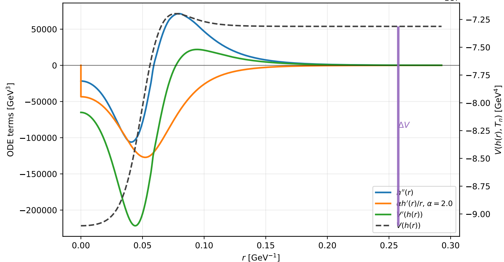
Example F7: bounce equation terms at T_n = 71.17 GeV
