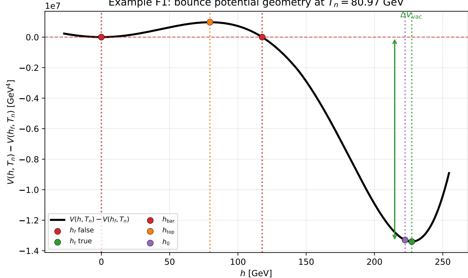
Example F1: bounce potential geometry at T_n = 80.97 GeV
