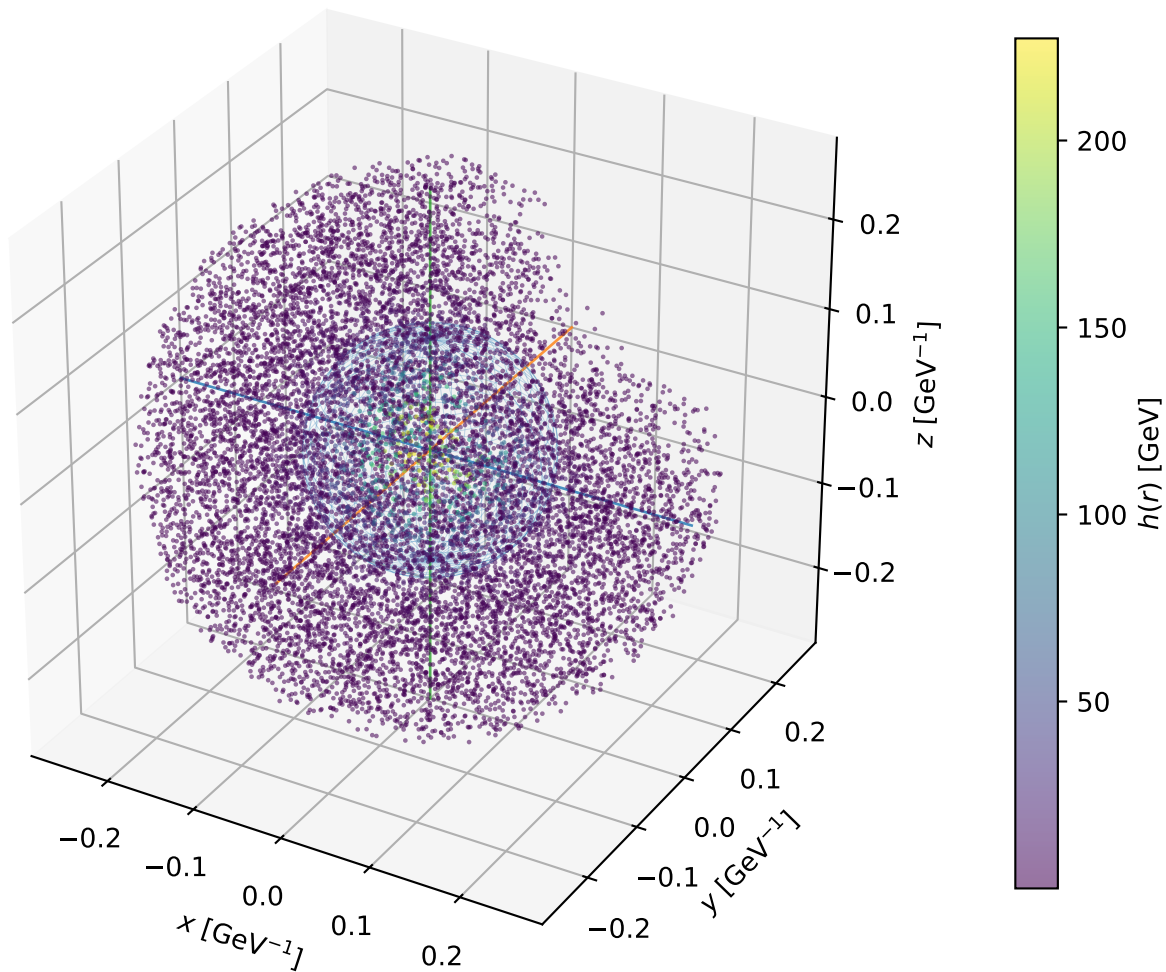
Example F5: 3D bubble profile at T_n = 80.97 GeV
