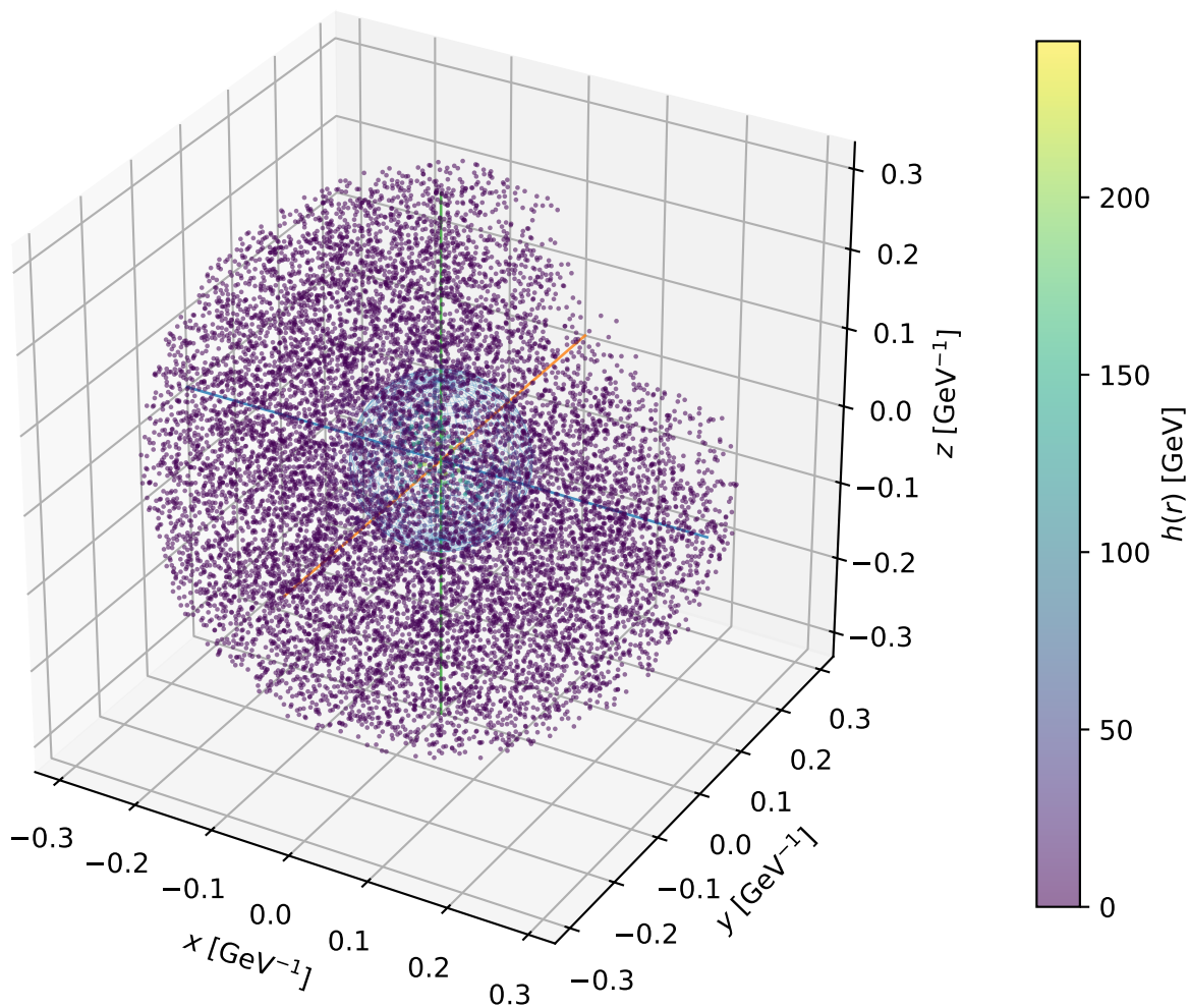
Example F5: 3D bubble profile at T_n = 43.95 GeV
