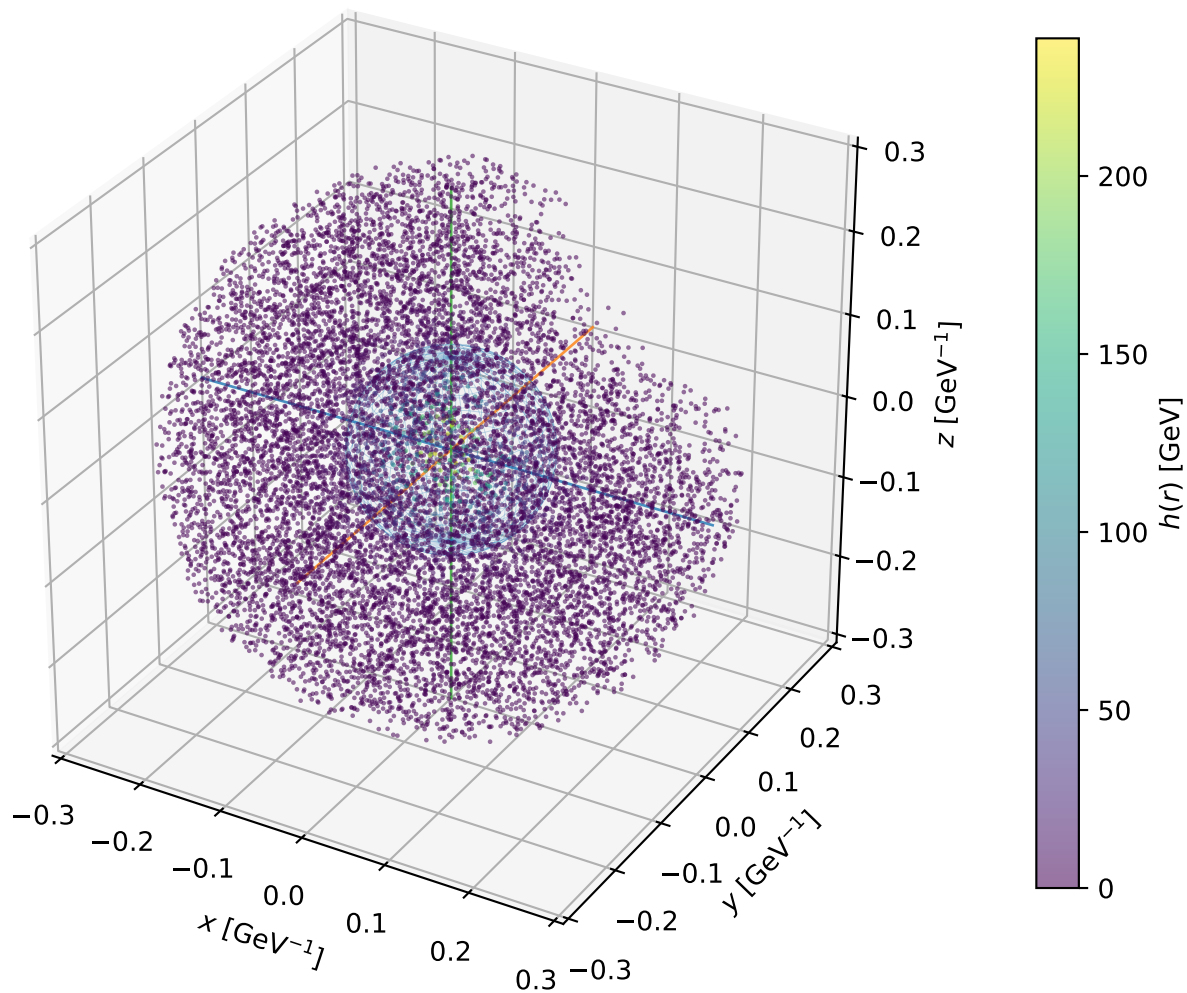
Example F5: 3D bubble profile at T_n = 63.1 GeV
