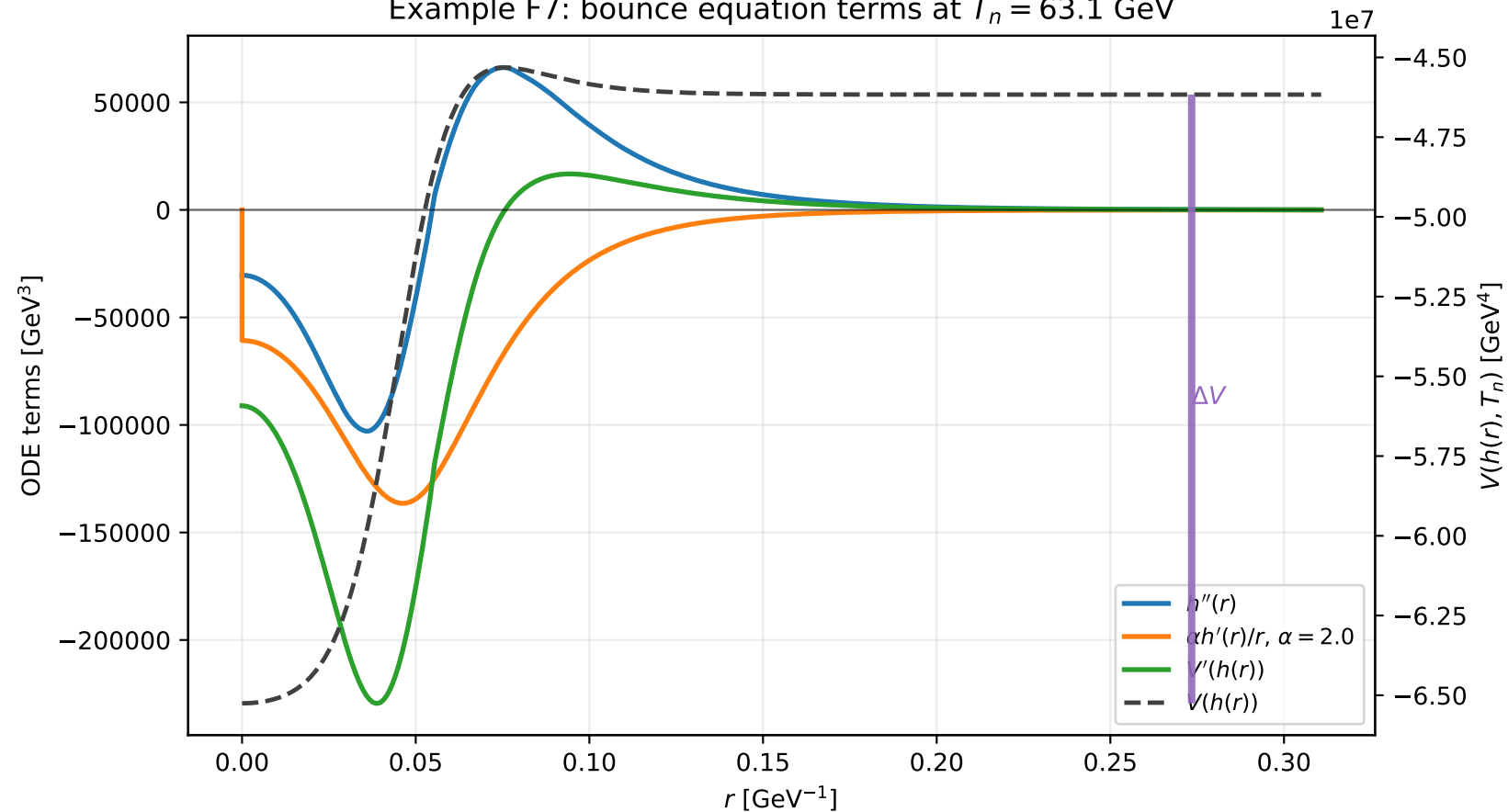
Example F7: bounce equation terms at T_n = 63.1 GeV
