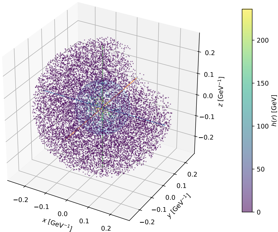
Example F5: 3D bubble profile at T_n = 68.62 GeV
