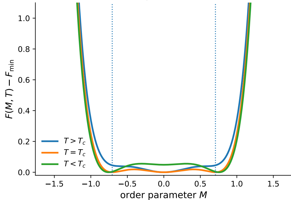
(a) Coexisting minima and barrier
