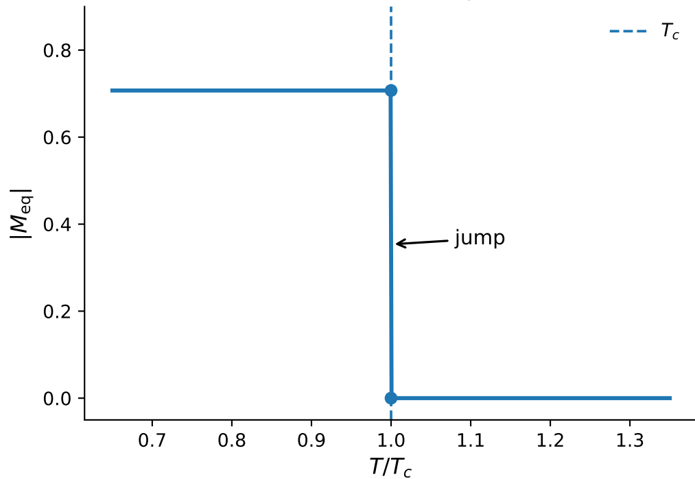
(b) Discontinuous order parameter
