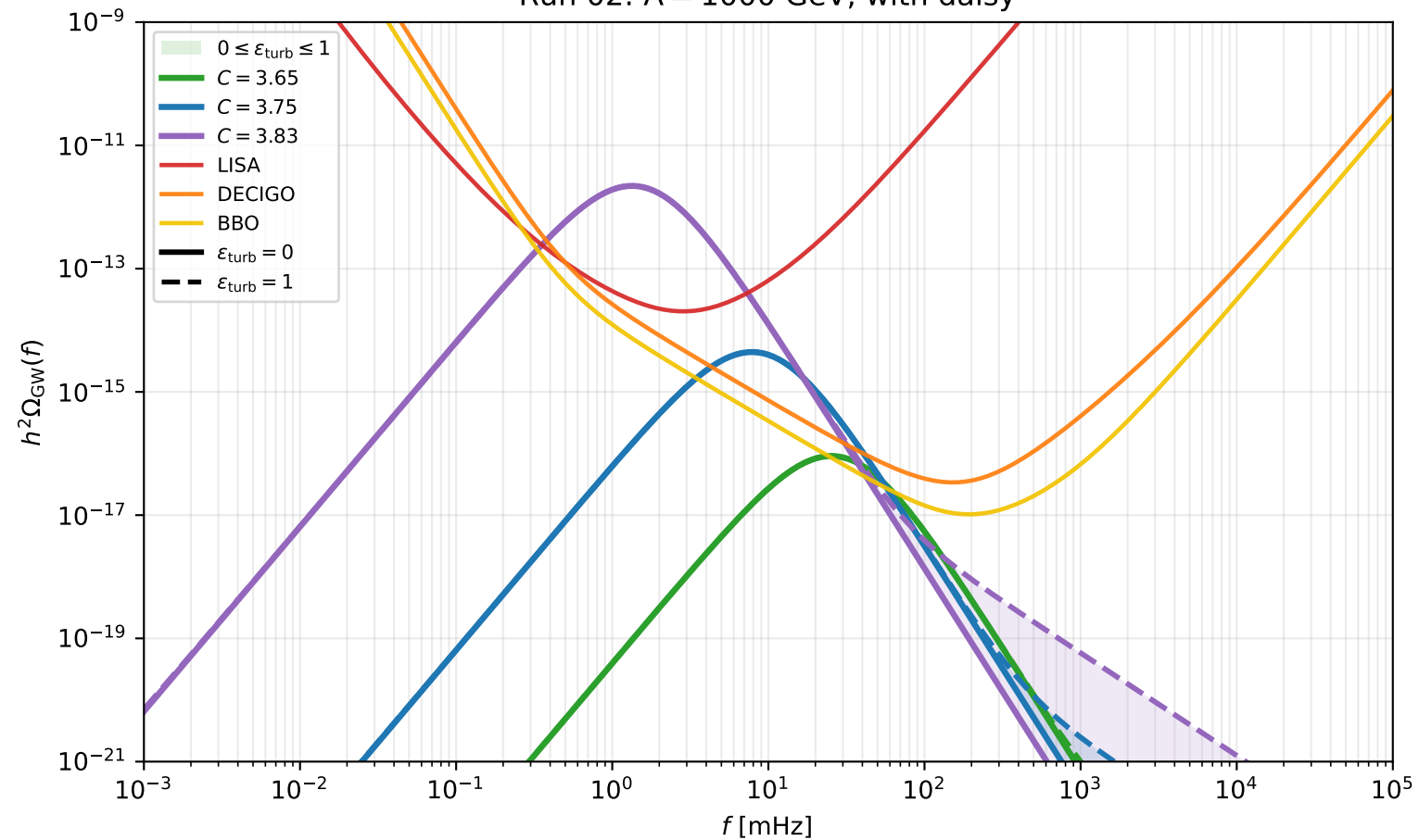
Run 02: \Lambda = 1000 GeV, with daisy
