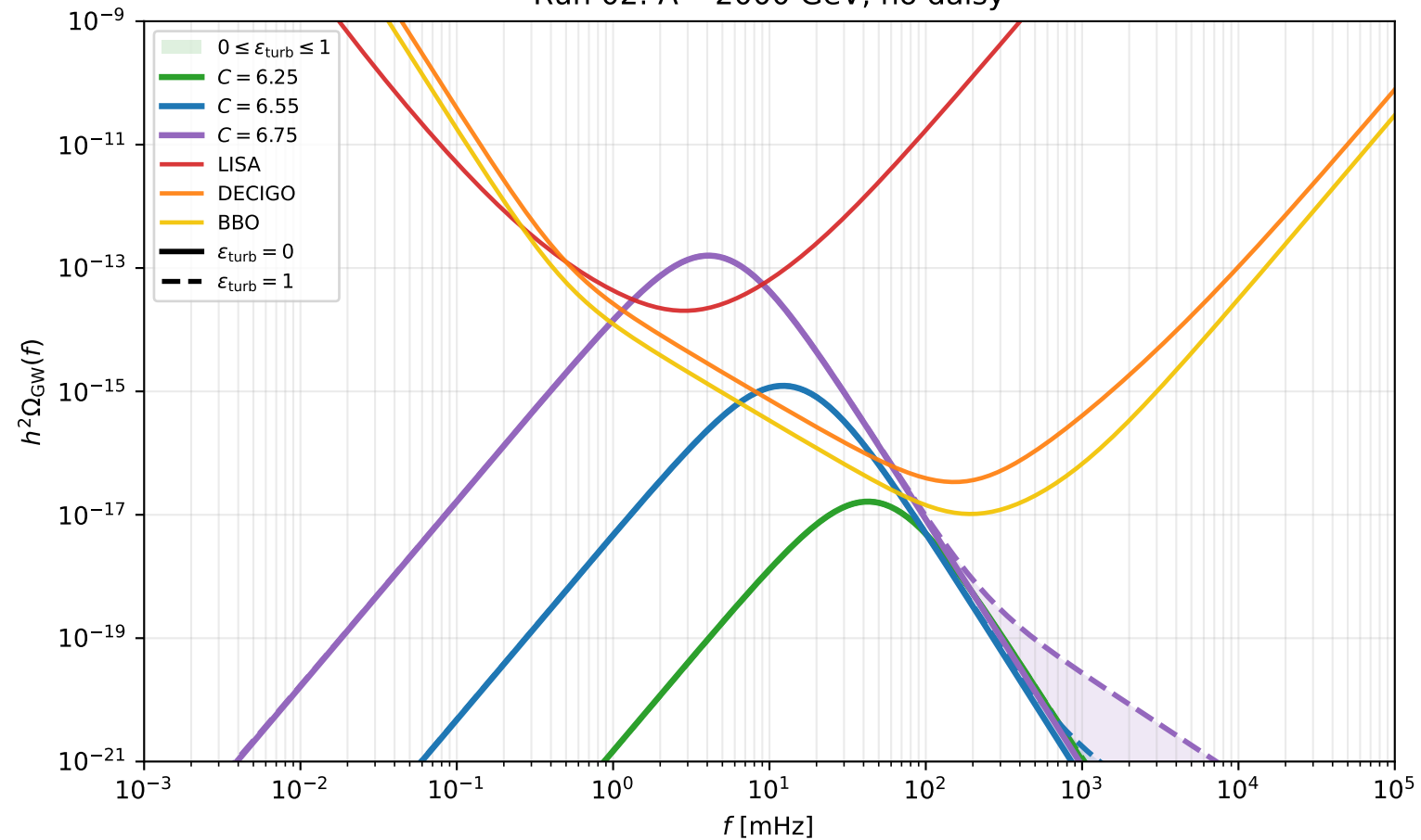
Run 02: \Lambda = 2000 GeV, no daisy
