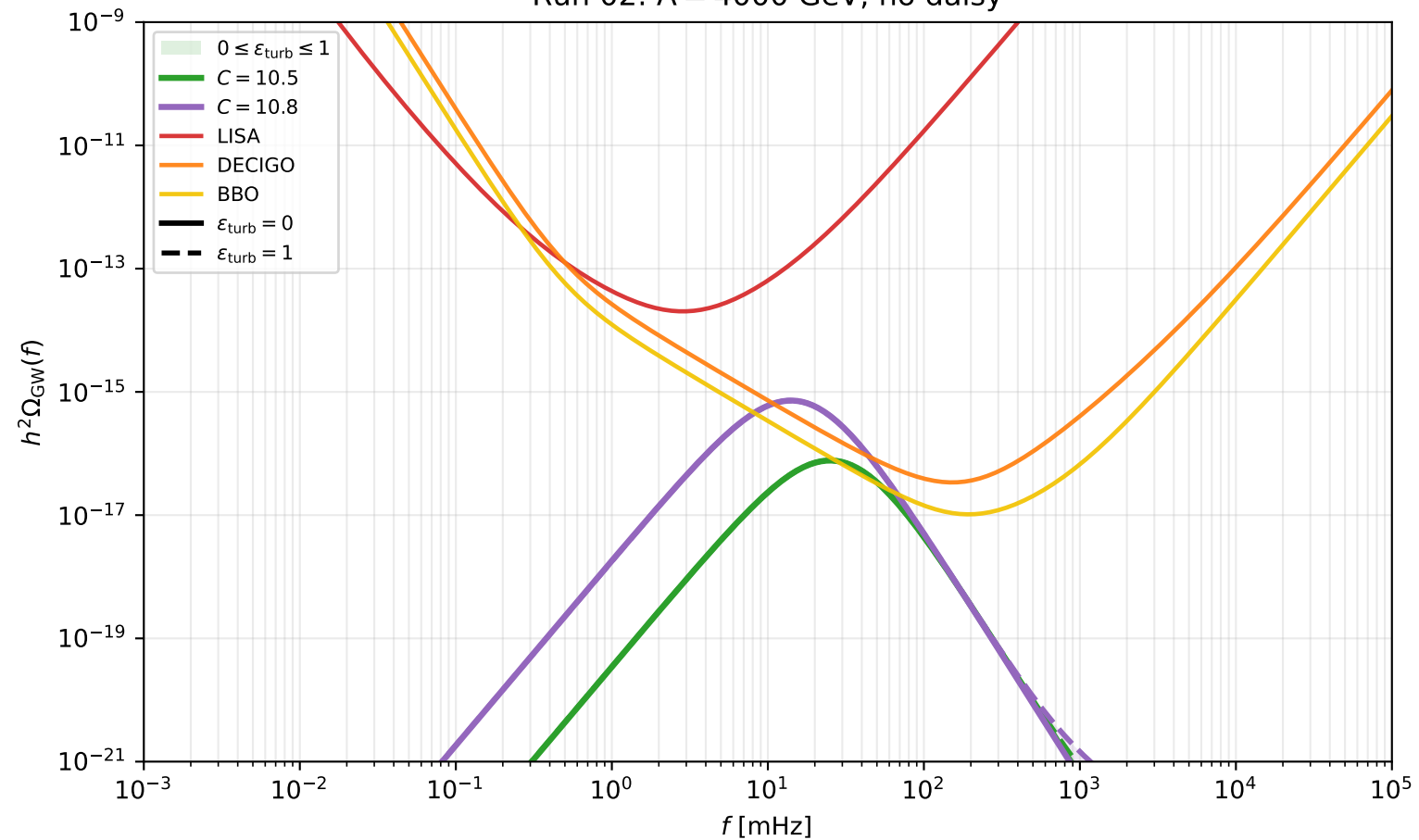
Run 02: \Lambda = 4000 GeV, no daisy
