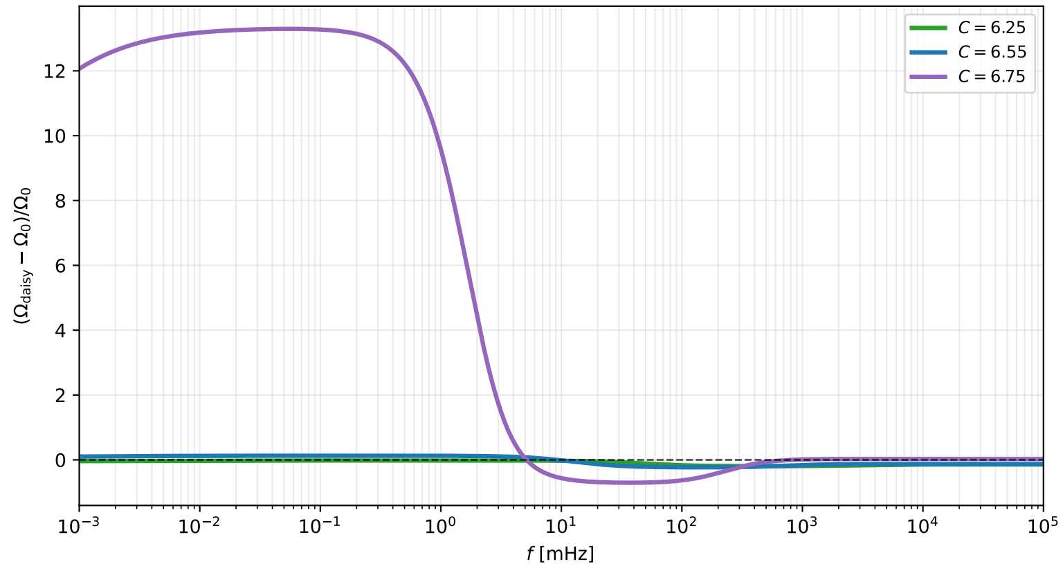
Run 02: relative daisy effect, \Lambda = 2000 GeV
