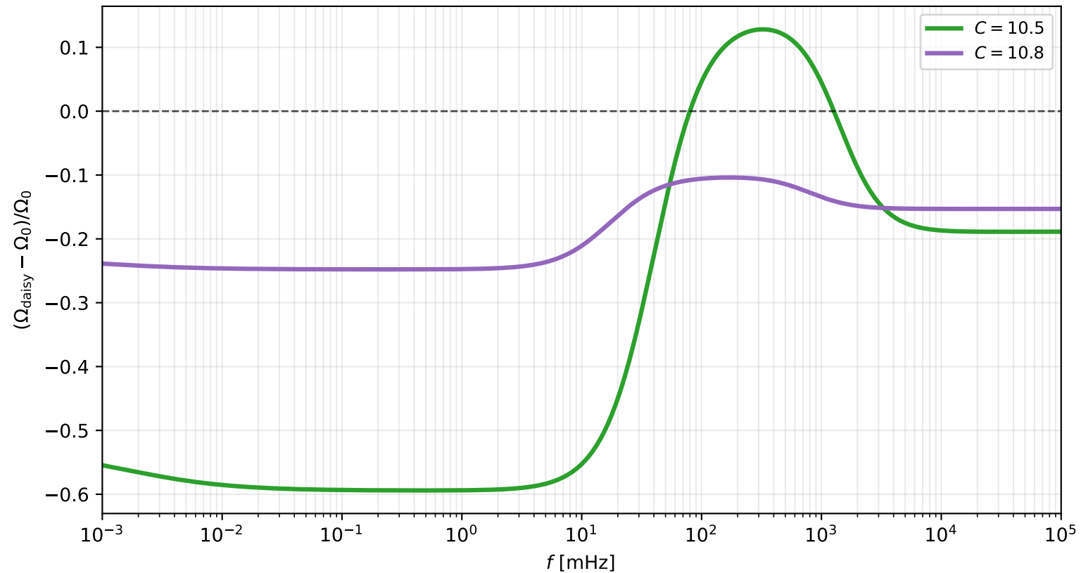
Run 02: relative daisy effect, \Lambda = 4000 GeV
