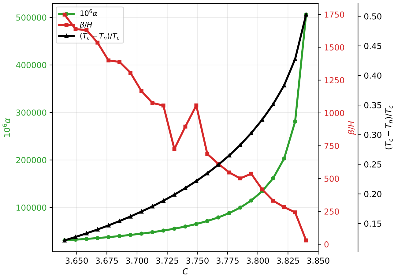
Run 03: \Lambda = 1000 GeV, no daisy
