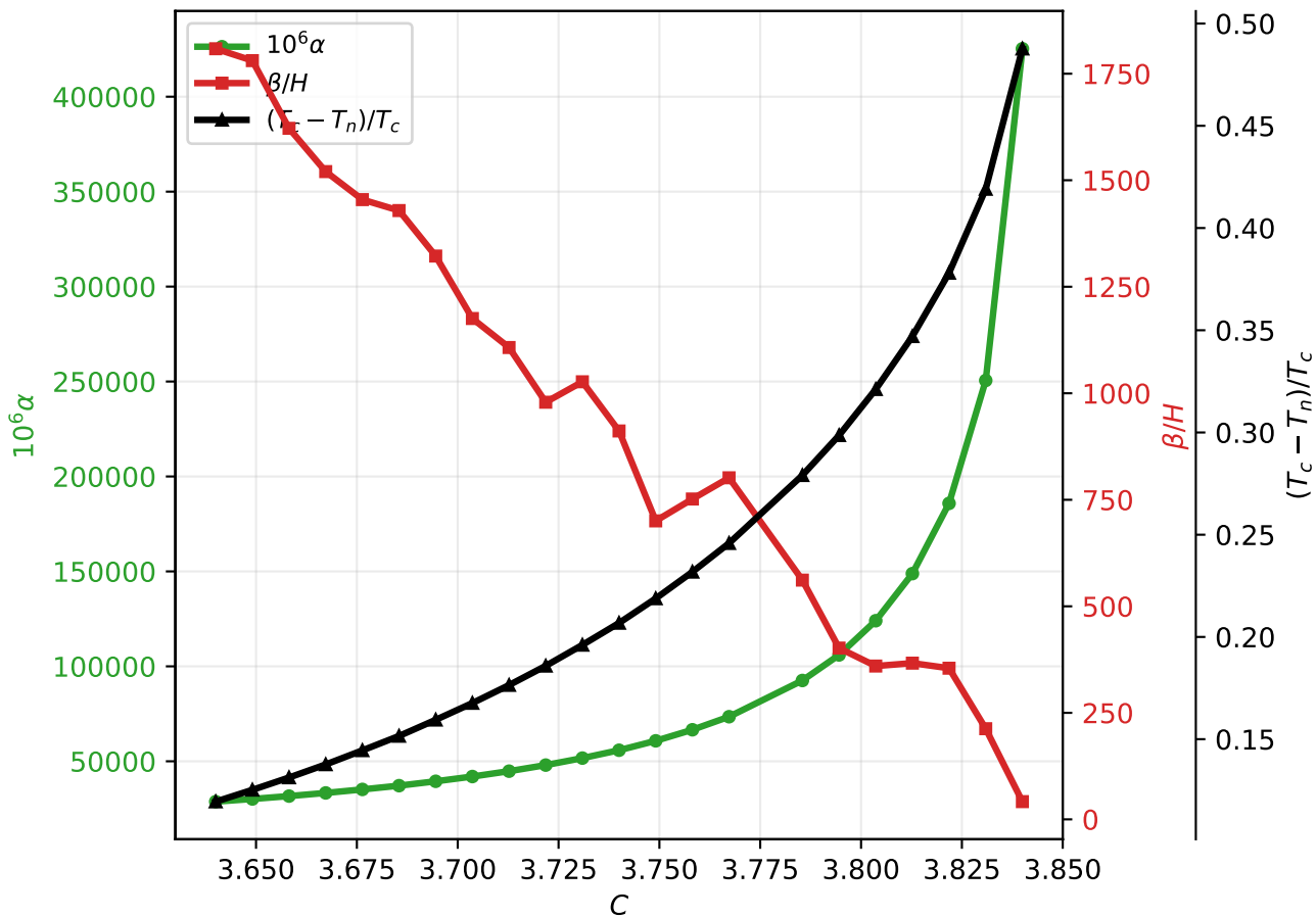
Run 03: \Lambda = 1000 GeV, with daisy
