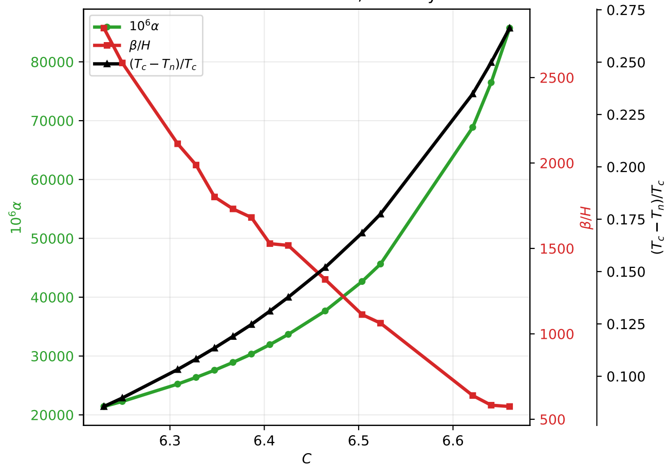
Run 03: \Lambda = 2000 GeV, no daisy
