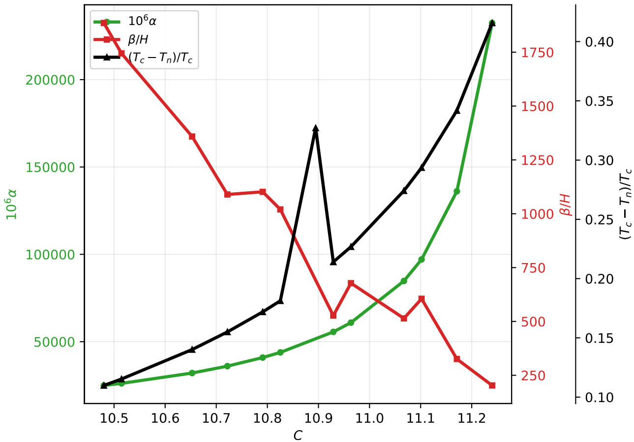
Run 03: \Lambda = 4000 GeV, with daisy
