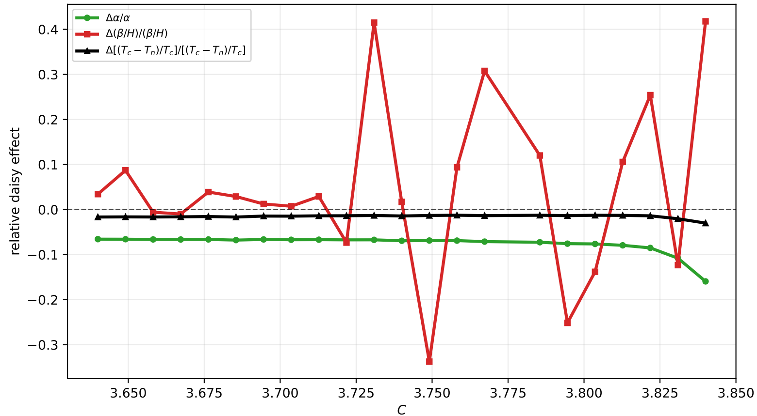
Run 03: relative daisy effect, \Lambda = 1000 GeV
