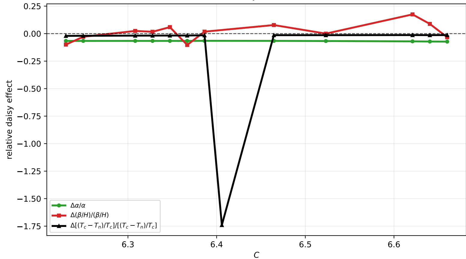
Run 03: relative daisy effect, \Lambda = 2000 GeV
