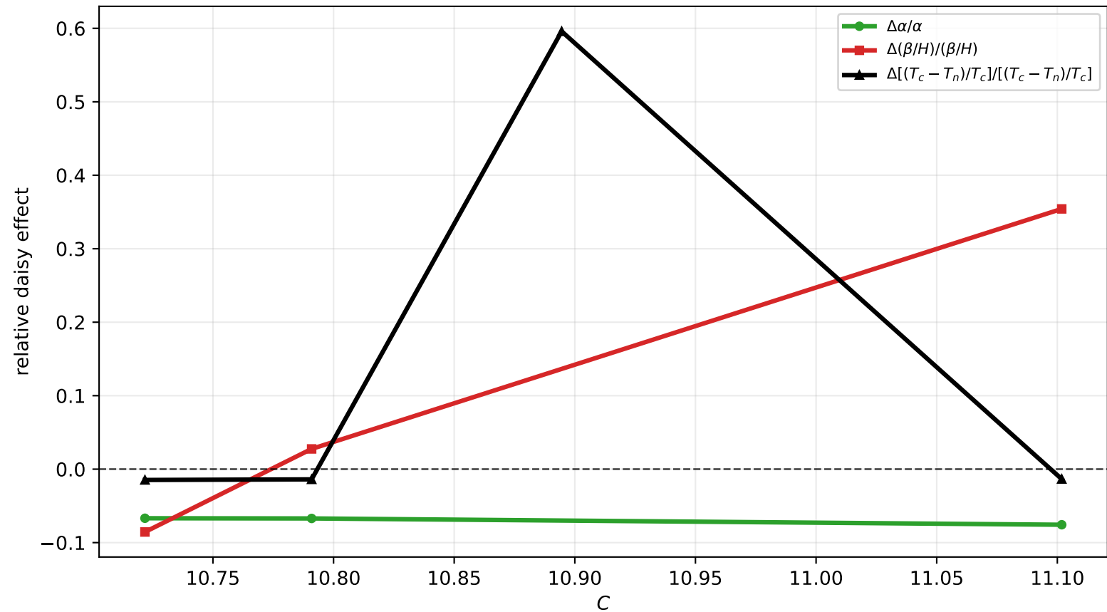
Run 03: relative daisy effect, \Lambda = 4000 GeV
