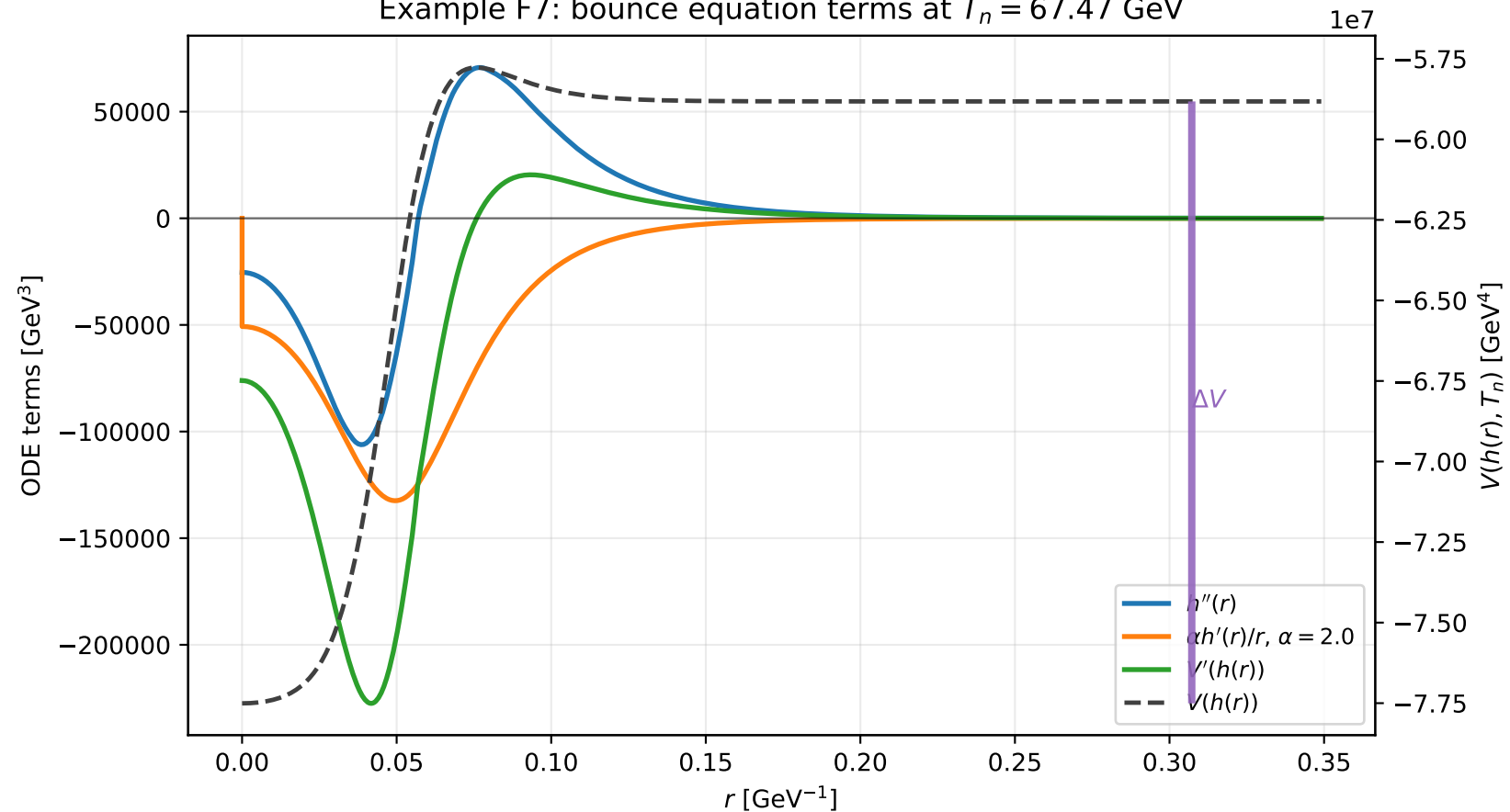
Example F7: bounce equation terms at T_n = 67.47 GeV
