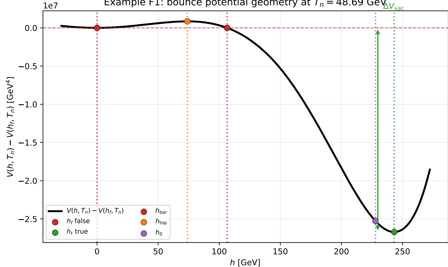
Example F1: bounce potential geometry at T_n = 48.69 GeV
