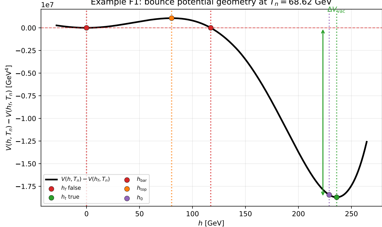
Example F1: bounce potential geometry at T_n = 68.62 GeV
