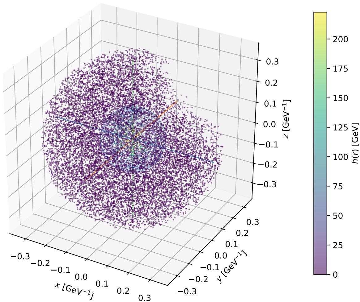
Example F5: 3D bubble profile at T_n = 85.16 GeV
