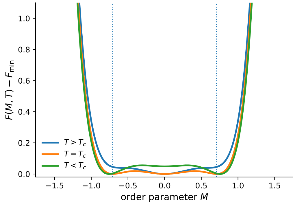
(a) Coexisting minima and barrier
