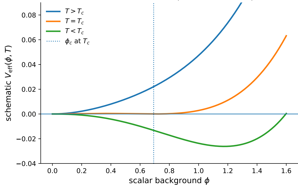
Schematic first-order finite-temperature effective potential
