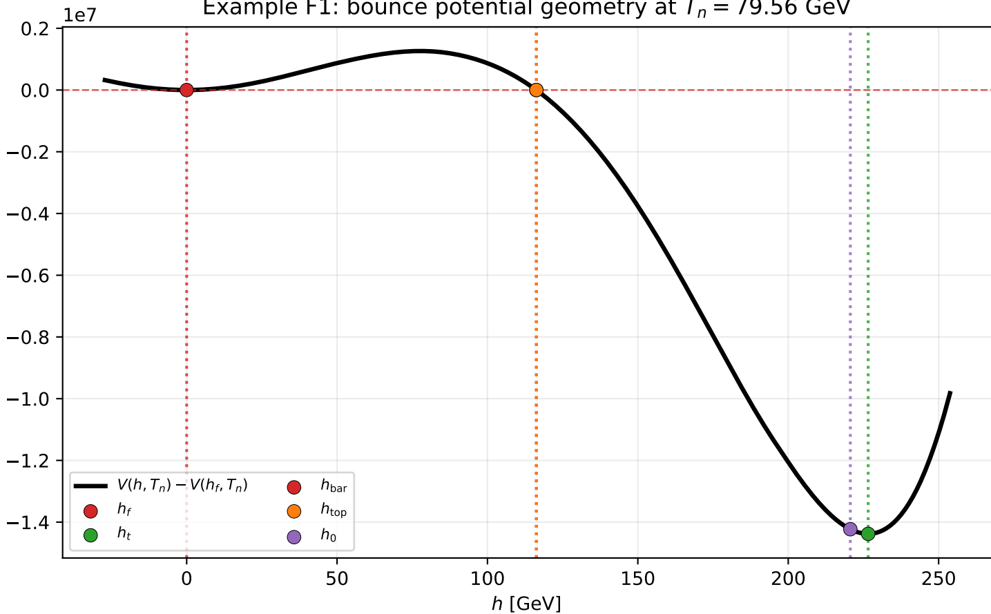
Example F1: bounce potential geometry at T_n = 79.56 GeV
