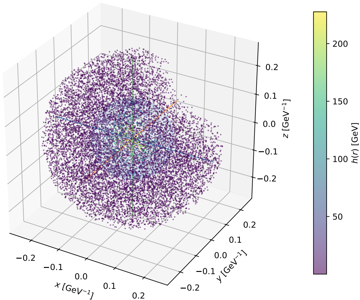
Example F5: 3D bubble profile at T_n = 79.69 GeV
