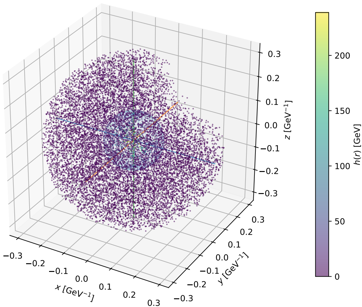
Example F5: 3D bubble profile at T_n = 62.02 GeV
