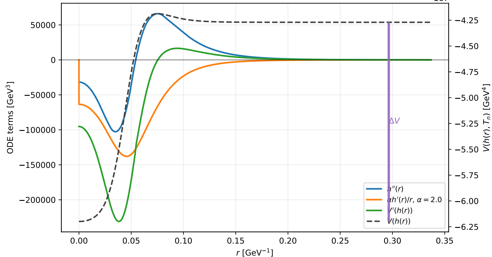
Example F7: bounce equation terms at T_n = 62.02 GeV
