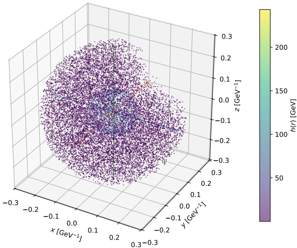
Example F5: 3D bubble profile at T_n = 47.65 GeV
