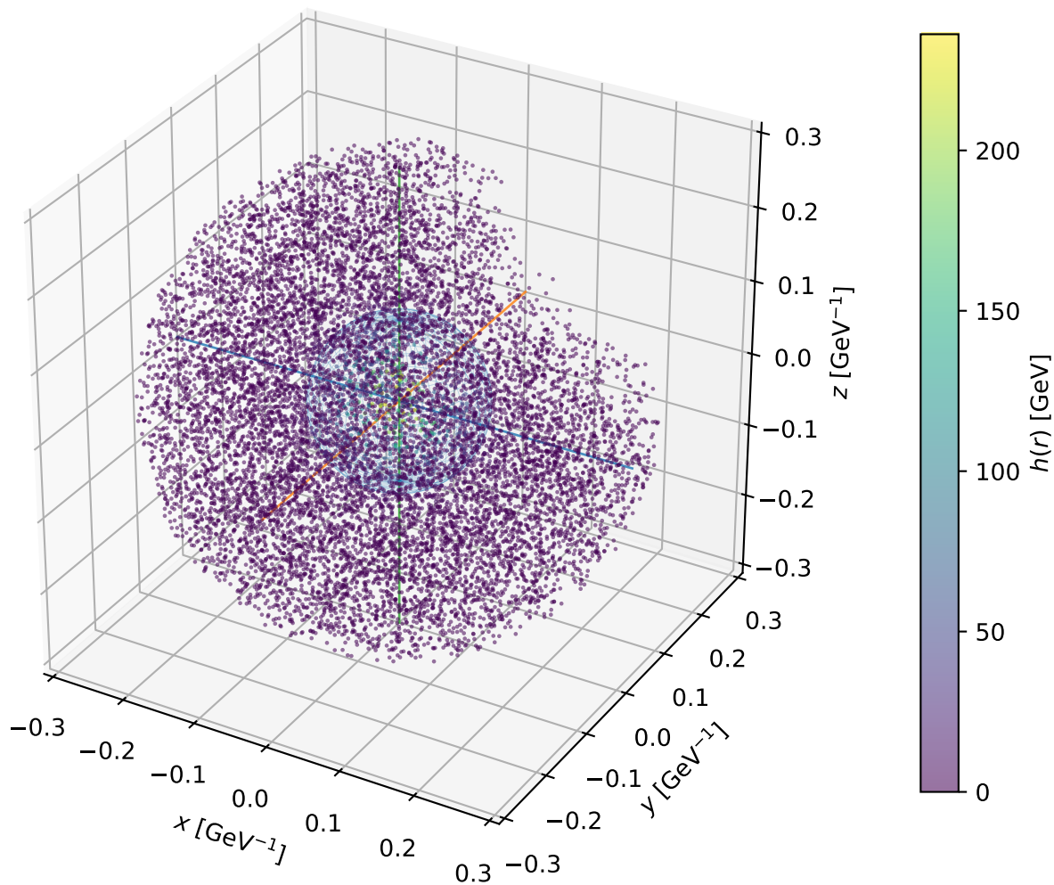
Example F5: 3D bubble profile at T_n = 67.48 GeV
